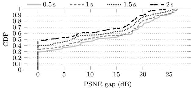
Figure 10: PSNR gap between the optimal scheduler and the FIFO scheduler. Positive gaps means that the PSNR of the optimal is greater than the one of the FIFO. We represent the CDF of the 168 transmissions.
