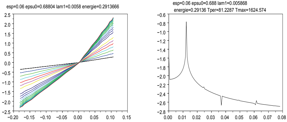
Figure 8: energy=0.29, 5 dof; left: configuration space; right:fft
