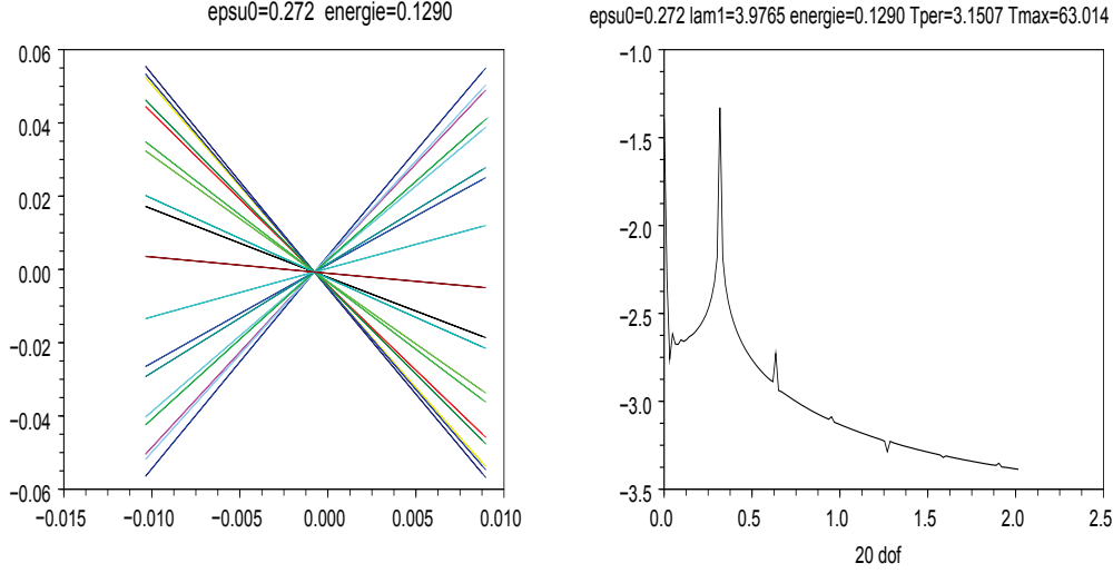
Figure 7: energy=0.129, 20 dof; left:in configuration space; right: fourier transform
