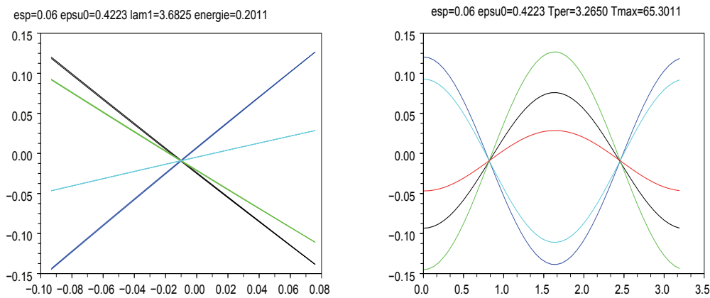
Figure 6: energy=0.2, 5 dof; left: configuration space; right:with respect to time
