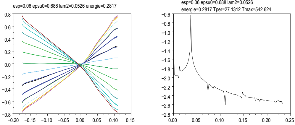
Figure 10: energy=0.28, 5 dof; left: configuration space; right:fft
