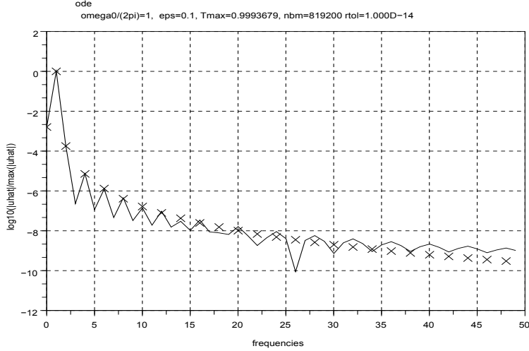
Figure 2: v_1, \log_{10} \left( \frac{|\widehat{u}_\varepsilon|}{\max |\widehat{u}_\varepsilon|} \right)
