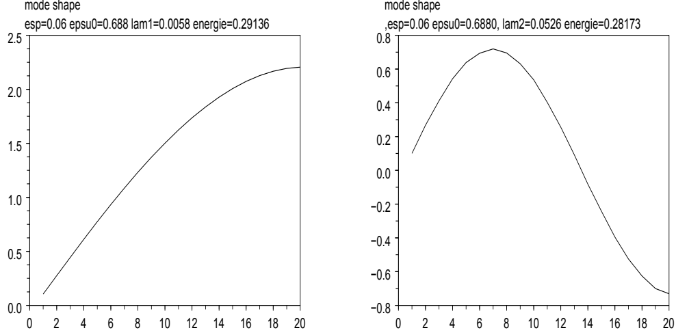
Figure 9: 20 dof; left:energy 0.29 mode 1; right: energy 0.28, mode 2
